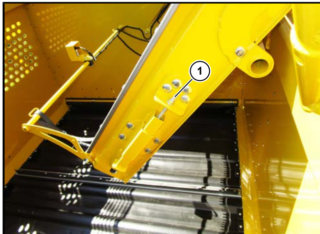
(1) Verleseband Spanner links
